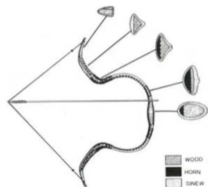
Sketch of composite bow with cross sectional views of materials. The sinew is in tension and horn in compression
